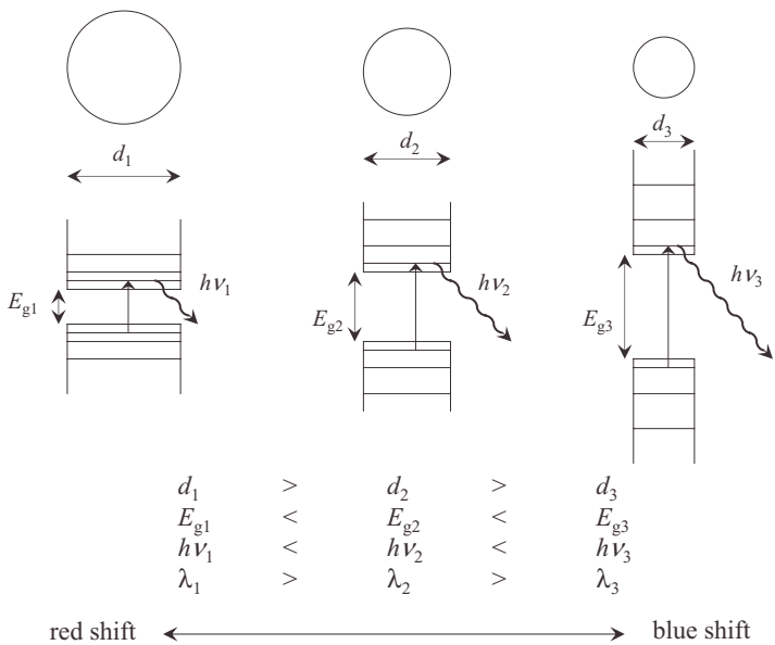
Figure 10.12. Schematic illustration of nanoparticles in optical sensory applications.
