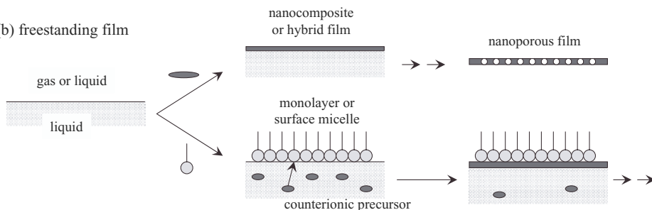
Figure 11.6. Different routes for the preparation of nanostructured films by sol–gel process.
