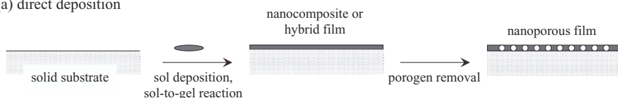
(a) direct deposition
