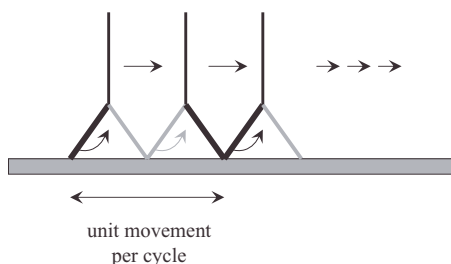
Figure 14.7. Unit operation: walking.
