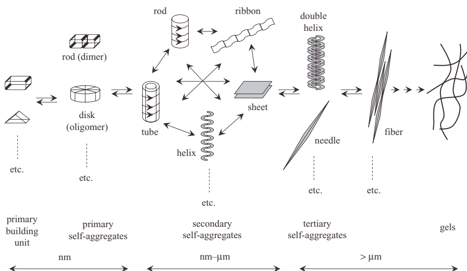
Figure 7.1. General scheme for bio-mimetic self-assembly.
