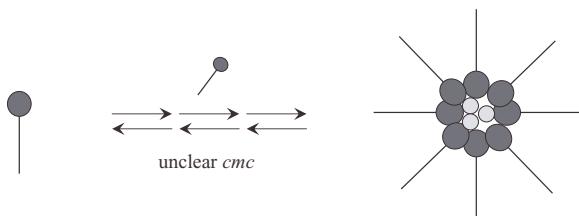
Figure 4.13. Formation of reverse micelles.
