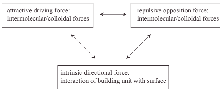
Figure 6.2. Force balance of interfacial self-assembly.
