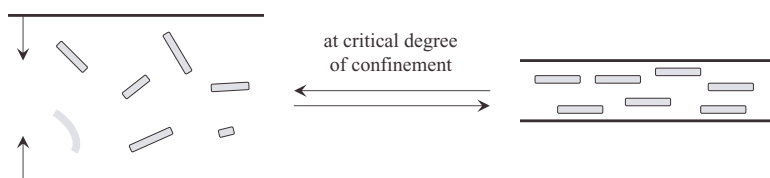
Figure 12.10. Molecular self-assembly within confined space.
