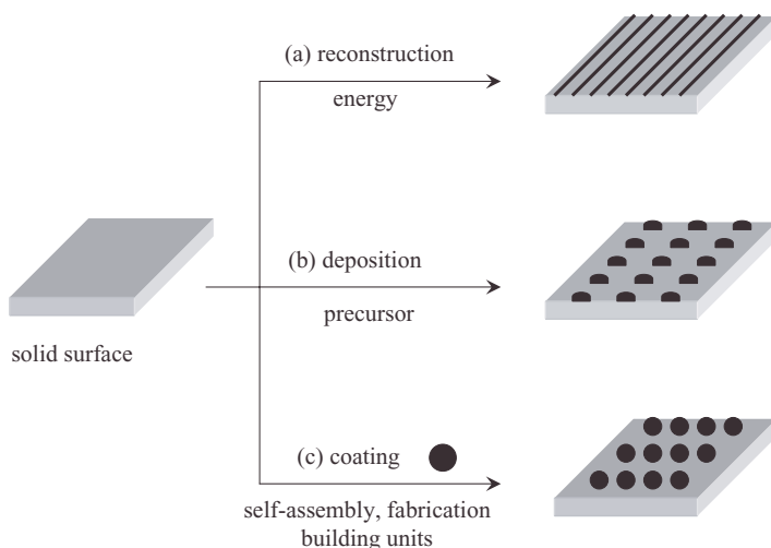
Figure 13.5. Unit fabrication: reconstruction, deposition, and coating.
