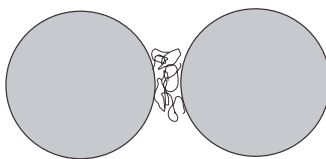
Figure 2.5. Schematic representation of attractive interaction between colloidal spheres via polymer bridging.
