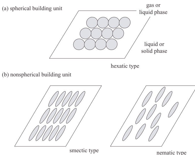
Figure 6.6. Typical packing of (a) spherical and (b) nonspherical nonamphiphiles at interfaces.
