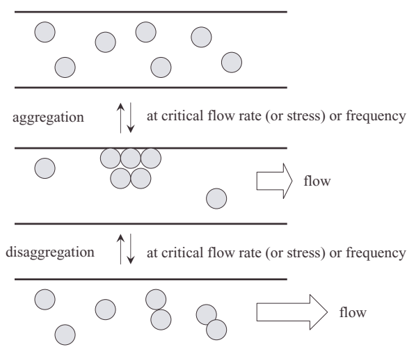
Figure 12.4. Self-assembly of colloidal particles under flow.
