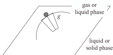
Figure 6.4. Two different types of amphiphile packing at interfaces.
