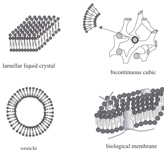
Figure 4.4. Schematic representation of different types of bilayers.
