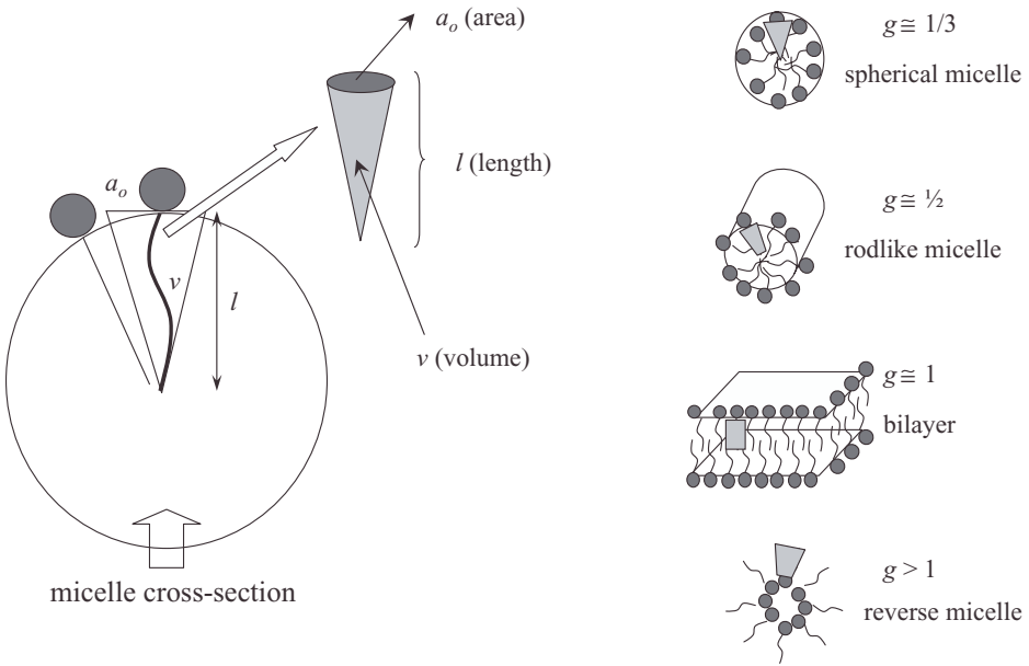
Figure 3.8. Surfactant (or micelle) packing parameter: g = v/a_o \cdot l .
